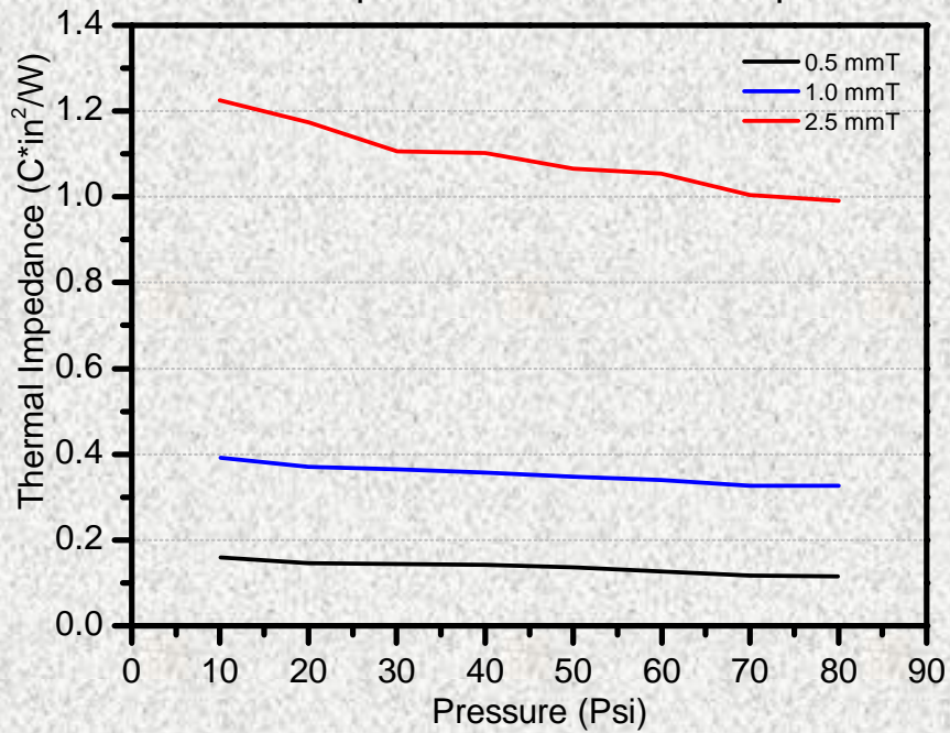
Thermal Impedance of OP-7400 Spec 01
