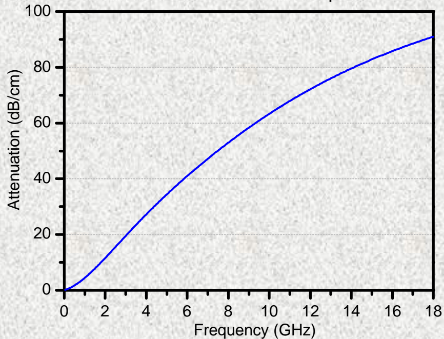
Attenuation of OP-7400 Spec01
